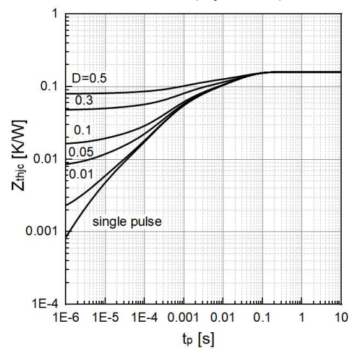
Fig 18. Transient thermal impedance of IGBT
